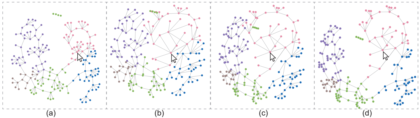
Fig. 5. Convergence of our method, where we perform our fisheye zoom at the focal point marked by a cursor using our structure-based, readability-based, and temporal constraints. (a) Input layout, and (b)-(d) results after 10, 20, and 30 iterations, respectively.
