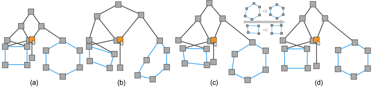
Fig. 3. Structure-based constraints: (a) input layout; (b) result produced by the graphical fisheye; (c) result produced by our method using only the edge orientation constraints; and (d) result produced by our method further using the shape constraints with the edge orientation constraints.
