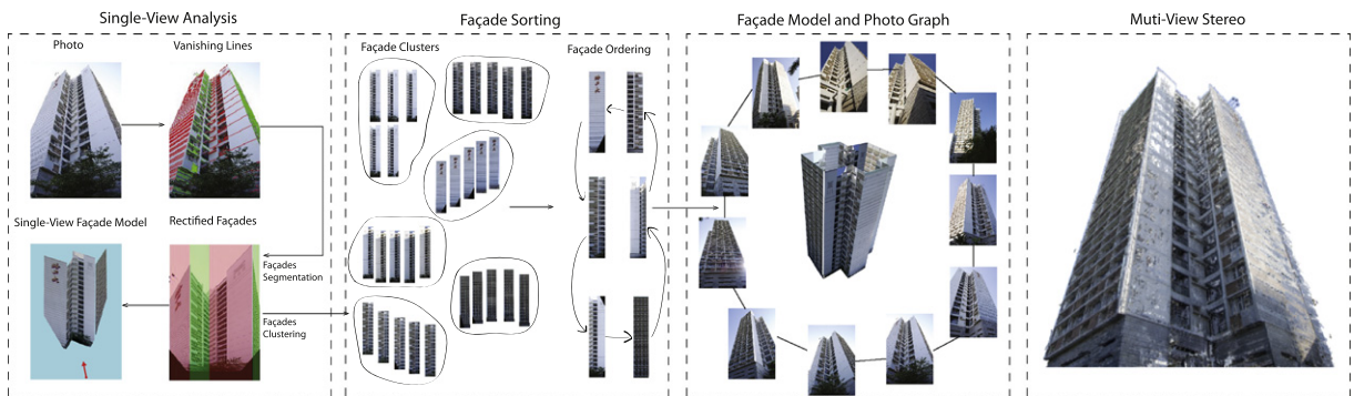
Fig. 3. From left to right: local geometry is estimated from each view, including vanishing points, segmented facades, and a local facade model; segmented facades are rectified and clustered, defining a facade graph which is analyzed to produce a simplified set of clusters; given this simplified facade graph, we generate a piece-wise planar facade model , compute a viewpoint for each image, and derive an image connectivity graph; this approximate model forms a good initialization to SfM and subsequent multi-view stereo methods.
