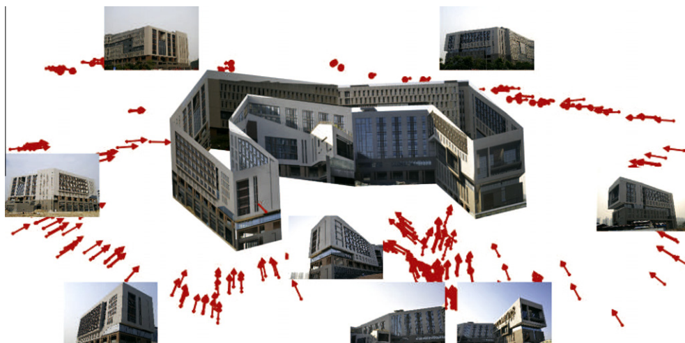
Fig. 2. A facade model produced by our technique applied to the collection summarized in Fig. 1 (shown here as thumbnails). The red arrows represent recovered camera poses. (For interpretation of the references to color in this figure legend, the reader is referred to the web version of this article.)
