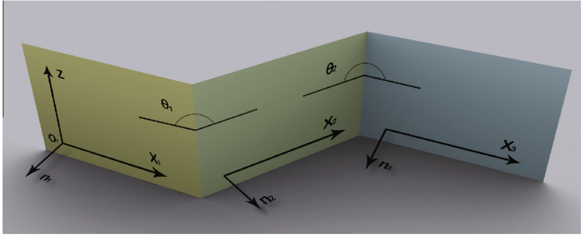
Fig. 6. Local coordinate defined by the left facade. The vector X_i corresponds to the horizontal VP for each facade, and Z corresponds to the direction of the vertical VP. The vector n_i represents the surface normal of facade i . \theta_1 and \theta_2 represent the interior angles between each pair of consecutive facades.
