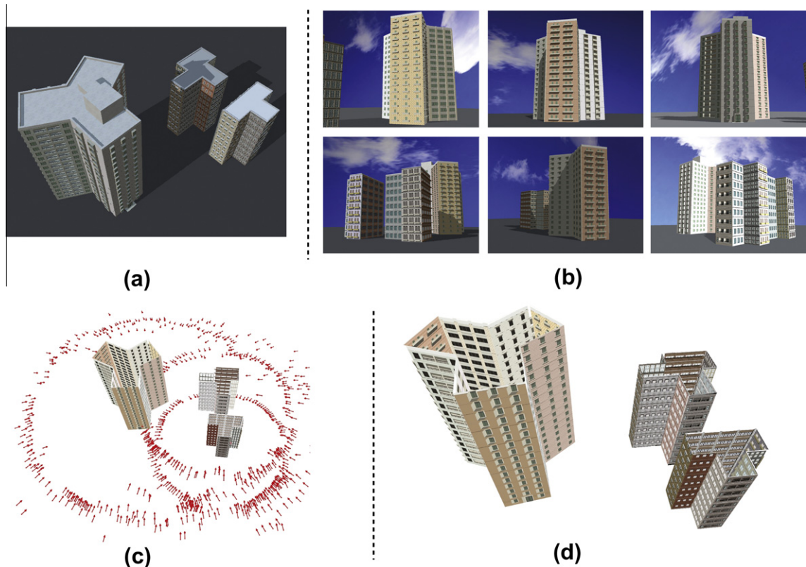
Fig. 15. Robustness to occlusions and multiple buildings. (a) A synthetic scene consisting of three buildings. (b) A sample of the simulated photos that contain occlusion and self-occlusions. (c) Recovered cameras. (d) Three piecewise-planar models that are reconstructed by our algorithm.
