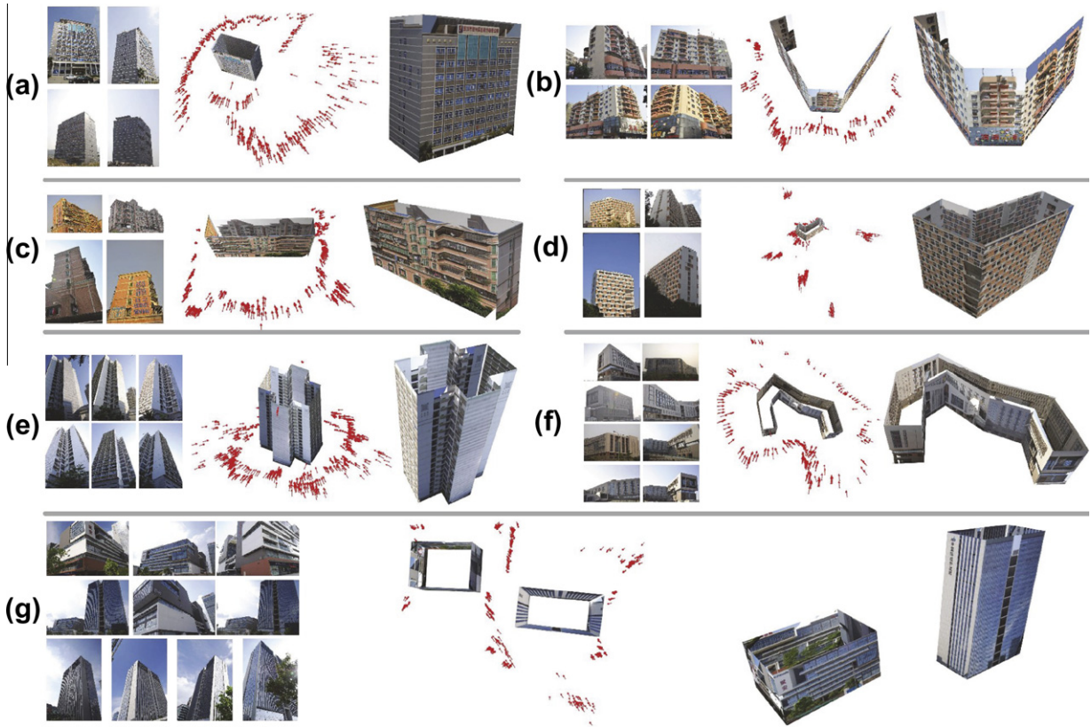
Fig. 11. Facade model results for our seven real-world datasets. Each dataset shows selected input images, initial cameras, and the output facade model.
