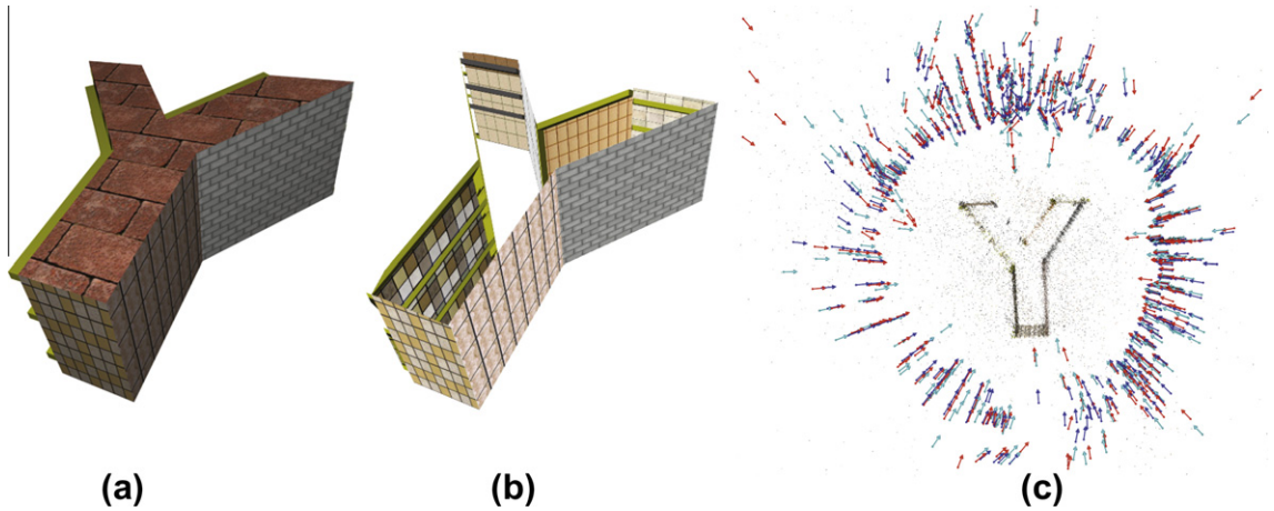
Fig. 13. Synthetic experiment: (a) Synthetic model used to generate the input photos. (b) Recovered facade-model. (c) SfM points and cameras from ground truth (blue), initial recovered positions (cyan) and refined positions (red). (For interpretation of the references to color in this figure legend, the reader is referred to the web version of this article.)
