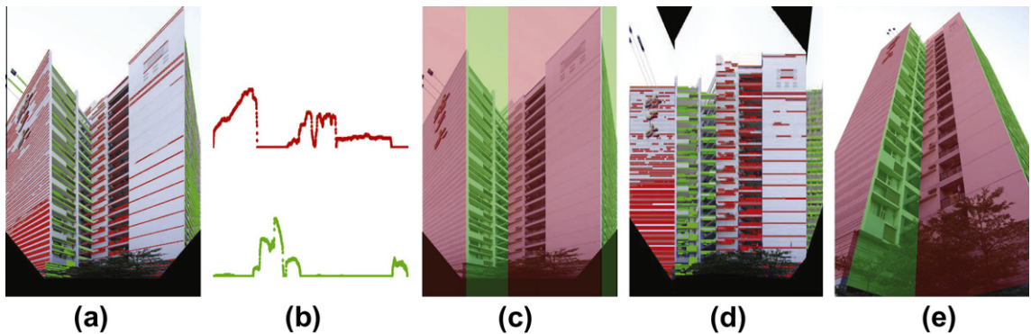
Fig. 4. Facade segmentation. (a) Rectified image with two groups of horizontal line segments according to two VP directions. (b) Histograms of the two horizontal line segments projected onto the x-axis of the image. (c) Segmentation along x-axis. (d) “Unwrapped” rectified image of segmented facades. (e) Segmented facades of the original image with top and bottom borders shown.
